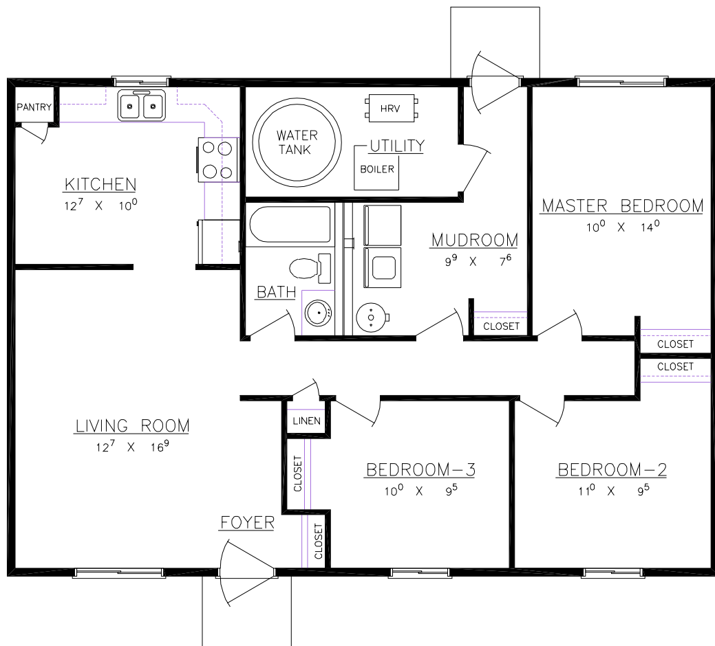
FLOOR PLAN
